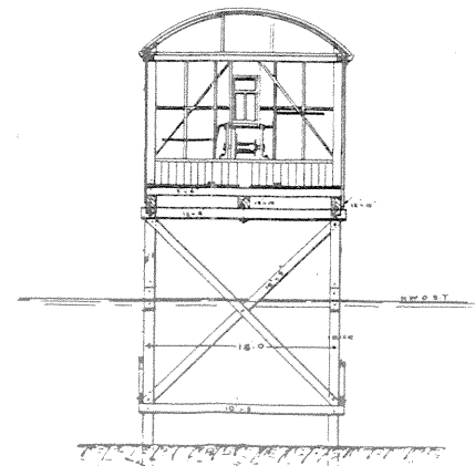
CROSS SECTION ON LINE A. B.
