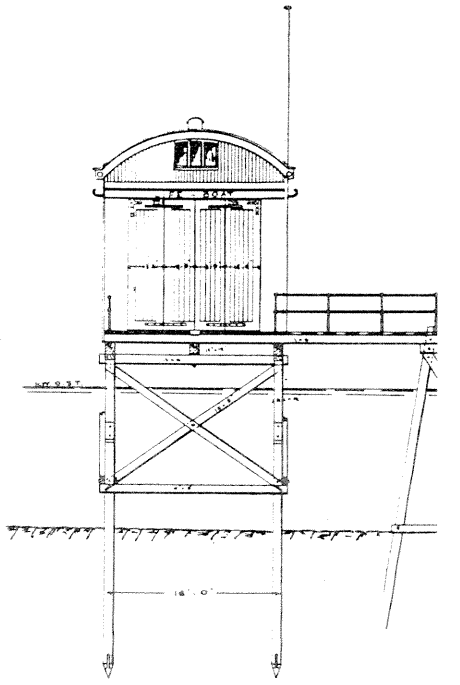
CROSS SECTION ON LINE C. D.
